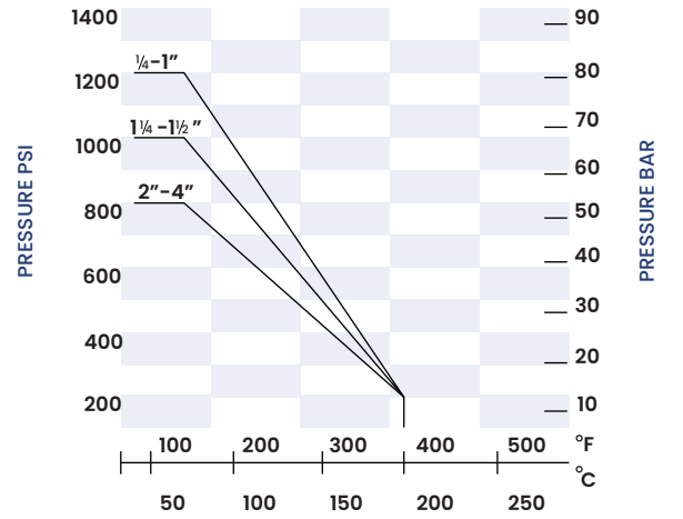
(PTFE) PRESSURE-TEMPERATURE RATING
